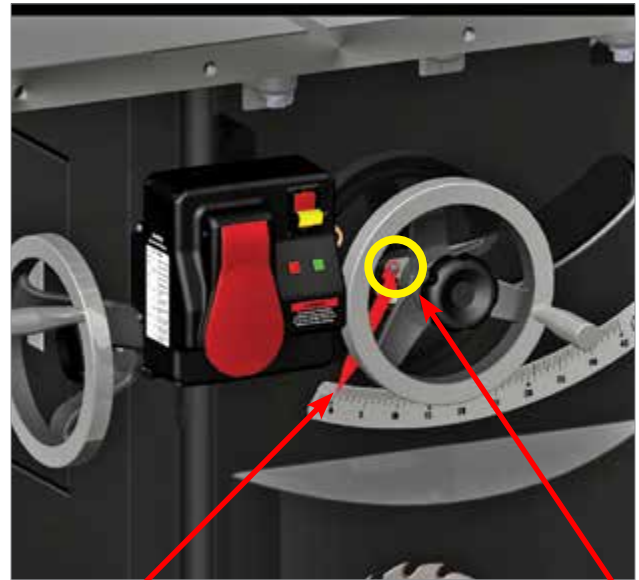
locking screw
